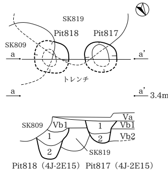
Pit818 (4J-2E15) Pit817 (4J-2E15)
