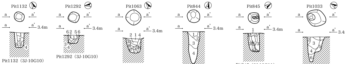
Pit1132 (3J-10G10) Pit1292 (3J-10G10) Pit1063 (3J-10G10,10H6) Pit844 (3J-10G11) Pit845 (3J-10G11) Pit1033 (3J-10G13・14)
